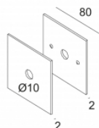
COVERSET S 80 204 80 80
