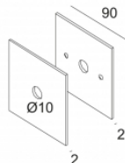
COVERSET S 90 204 90 90
