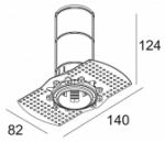
MOUNTING KIT SPY 39 TRIMLESS IN 24144 0050
